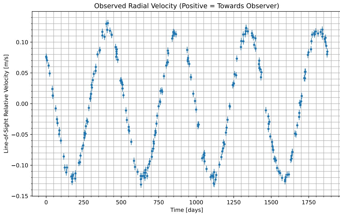
Figure 1: We have isolated the radial velocity of the host star due to the candidate planet. Data begins at UTC 2065-07-01/07:43. Positive values indicate the velocity at which the star is moving towards us; negative indicate the velocity at which it is moving away.
