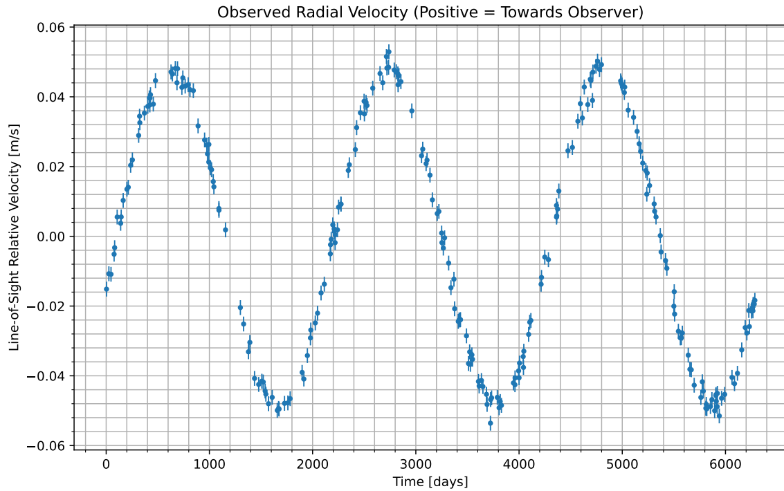
Figure 1: We have isolated the radial velocity of the host star due to the candidate planet. Data begins at UTC 2068-01-31/00:17. Positive values indicate the velocity at which the star is moving towards us; negative indicate the velocity at which it is moving away.
