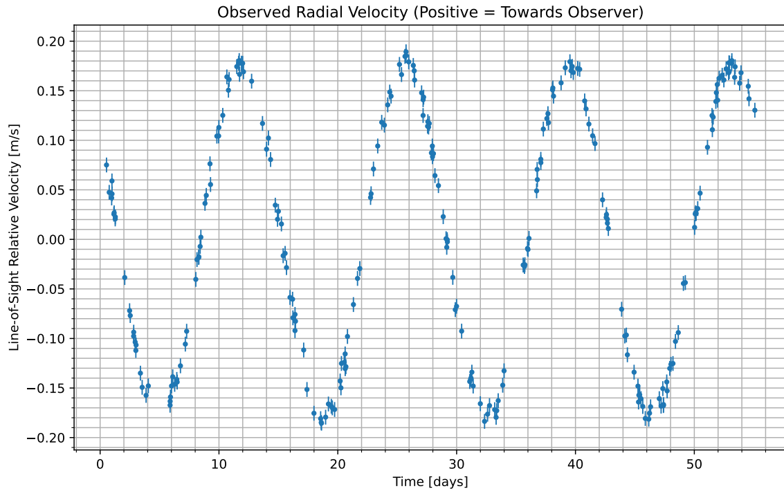
Figure 1: We have isolated the radial velocity of the host star due to the candidate planet. Data begins at UTC 2073-09-14/04:45. Positive values indicate the velocity at which the star is moving towards us; negative indicate the velocity at which it is moving away.
