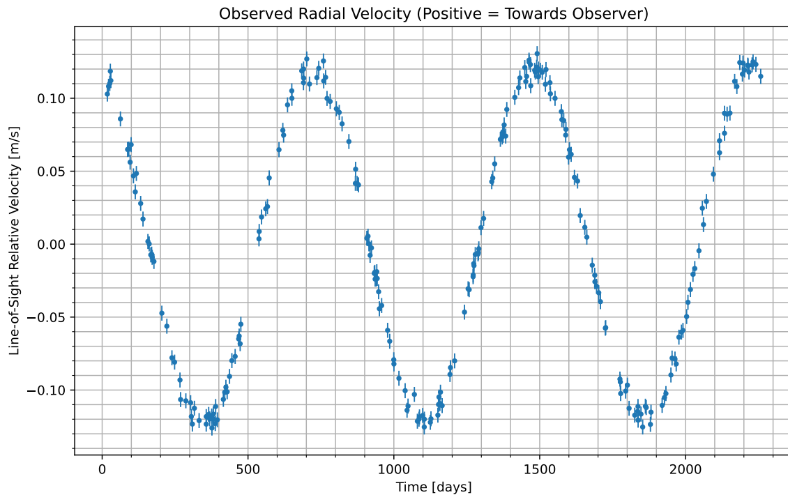
Figure 1: We have isolated the radial velocity of the host star due to the candidate planet. Data begins at UTC 2085-07-30/12:02. Positive values indicate the velocity at which the star is moving towards us; negative indicate the velocity at which it is moving away.
