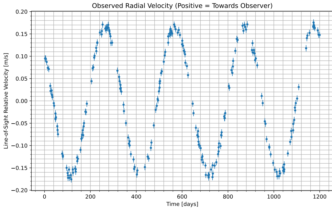
Figure 1: We have isolated the radial velocity of the host star due to the candidate planet. Data begins at UTC 2071-11-08/20:04. Positive values indicate the velocity at which the star is moving towards us; negative indicate the velocity at which it is moving away.
