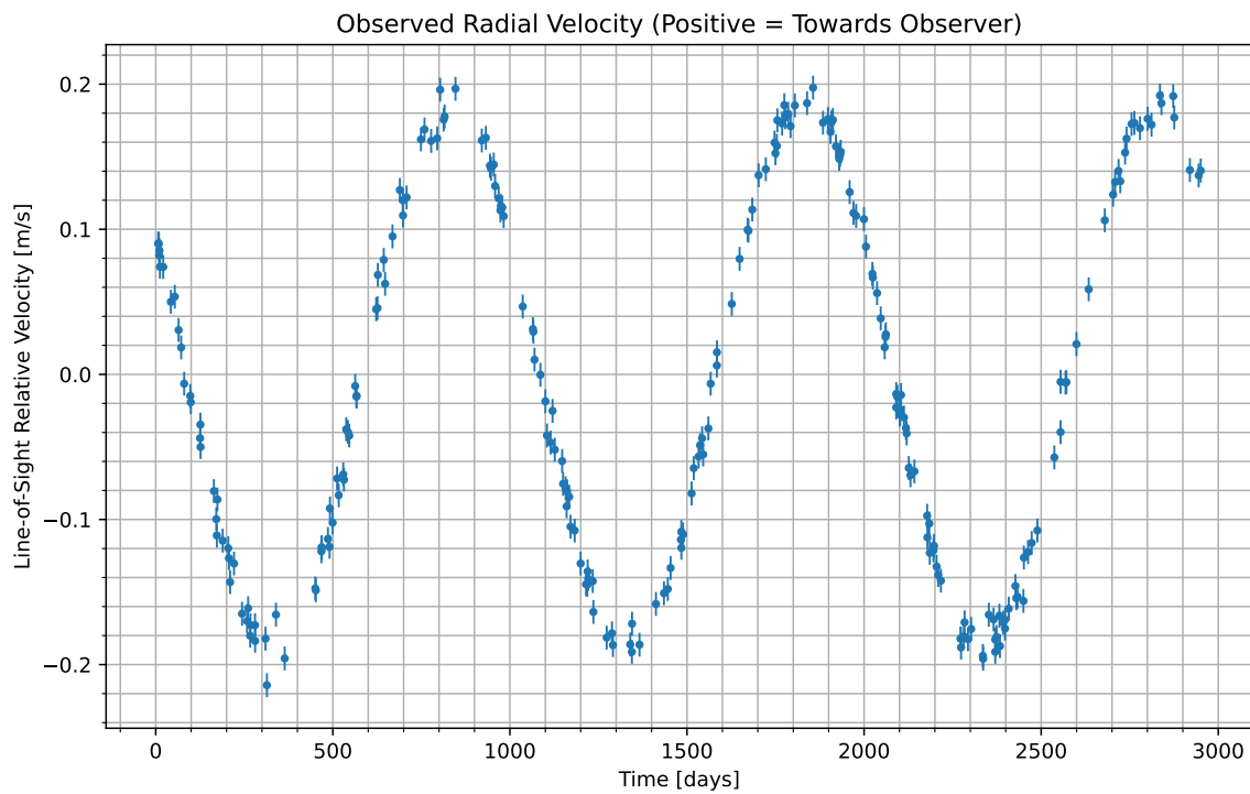
Figure 1: We have isolated the radial velocity of the host star due to the candidate planet. Data begins at UTC 2080-08-08/05:38. Positive values indicate the velocity at which the star is moving towards us; negative indicate the velocity at which it is moving away.
