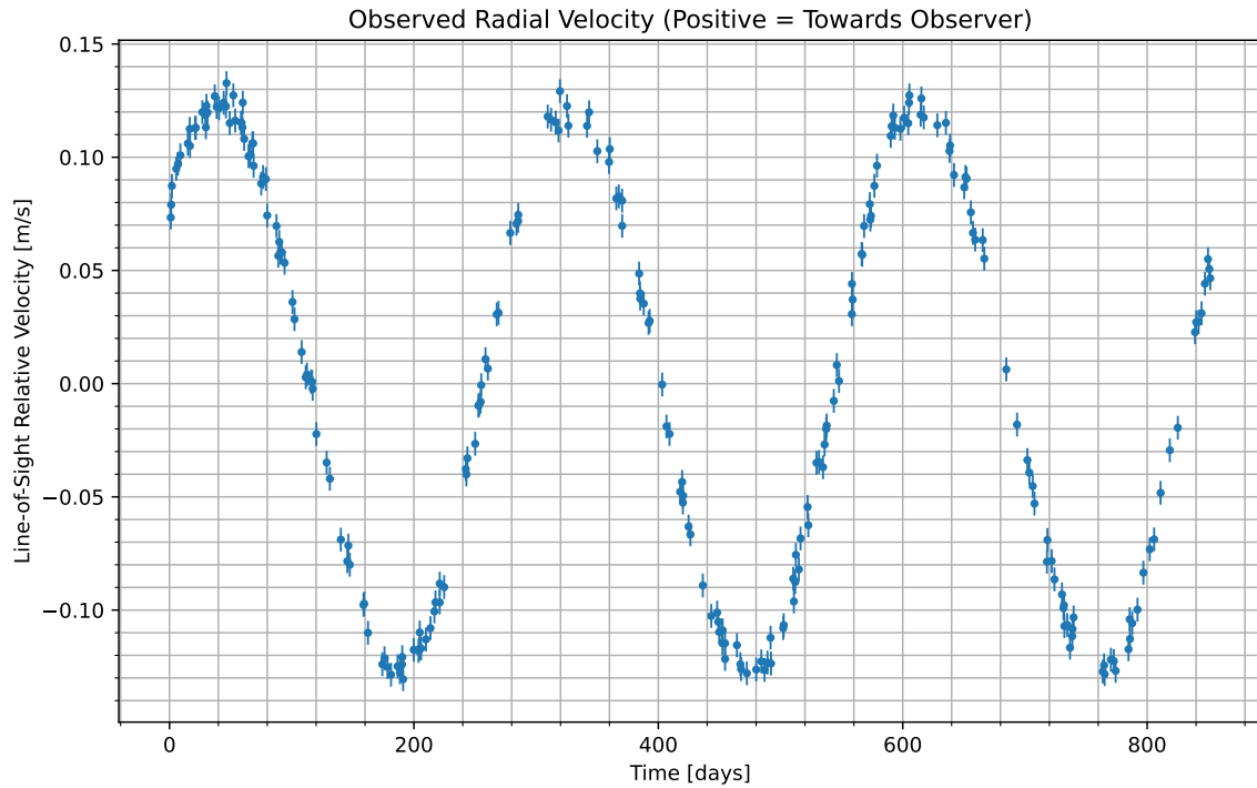
Figure 1: We have isolated the radial velocity of the host star due to the candidate planet. Data begins at UTC 2069-12-30/12:17. Positive values indicate the velocity at which the star is moving towards us; negative indicate the velocity at which it is moving away.
