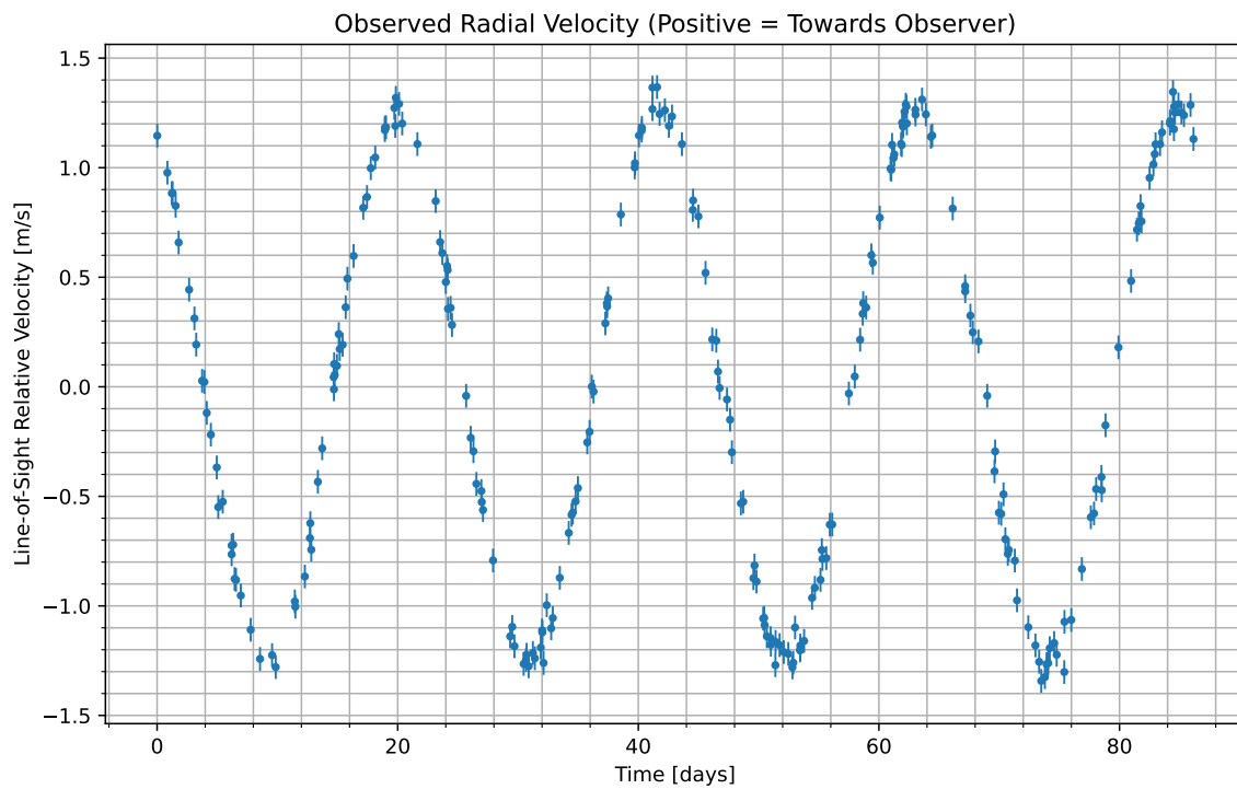
Figure 1: We have isolated the radial velocity of the host star due to the candidate planet. Data begins at UTC 2089-06-24/21:10. Positive values indicate the velocity at which the star is moving towards us; negative indicate the velocity at which it is moving away.
