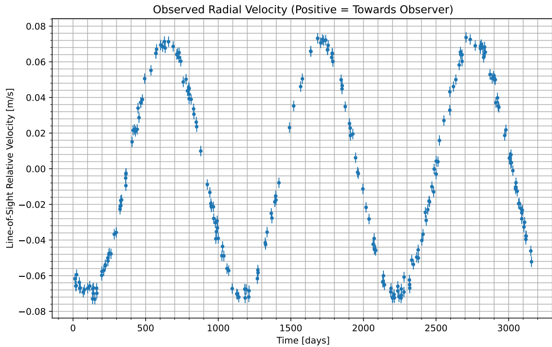
Figure 1: We have isolated the radial velocity of the host star due to the candidate planet. Data begins at UTC 2072-06-05/17:18. Positive values indicate the velocity at which the star is moving towards us; negative indicate the velocity at which it is moving away.
