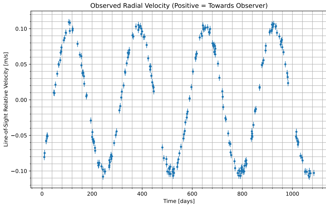
Figure 1: We have isolated the radial velocity of the host star due to the candidate planet. Data begins at UTC 2096-10-07/11:25. Positive values indicate the velocity at which the star is moving towards us; negative indicate the velocity at which it is moving away.
