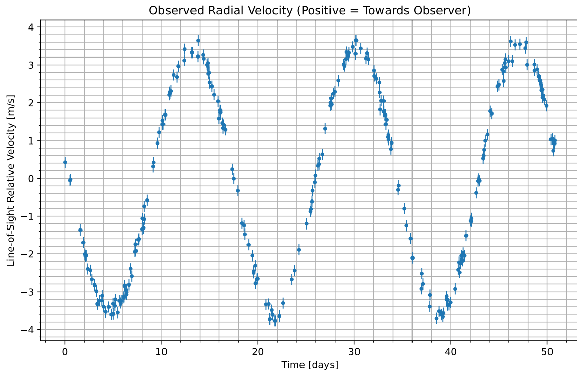
Figure 1: We have isolated the radial velocity of the host star due to the candidate planet. Data begins at UTC 2071-03-01/04:56. Positive values indicate the velocity at which the star is moving towards us; negative indicate the velocity at which it is moving away.
