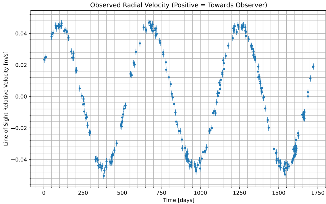
Figure 1: We have isolated the radial velocity of the host star due to the candidate planet. Data begins at UTC 2079-06-25/05:20. Positive values indicate the velocity at which the star is moving towards us; negative indicate the velocity at which it is moving away.
