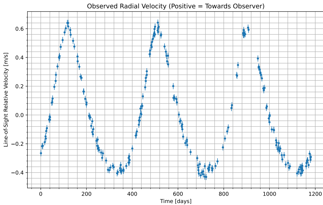
Figure 1: We have isolated the radial velocity of the host star due to the candidate planet. Data begins at UTC 2093-03-26/09:44. Positive values indicate the velocity at which the star is moving towards us; negative indicate the velocity at which it is moving away.
