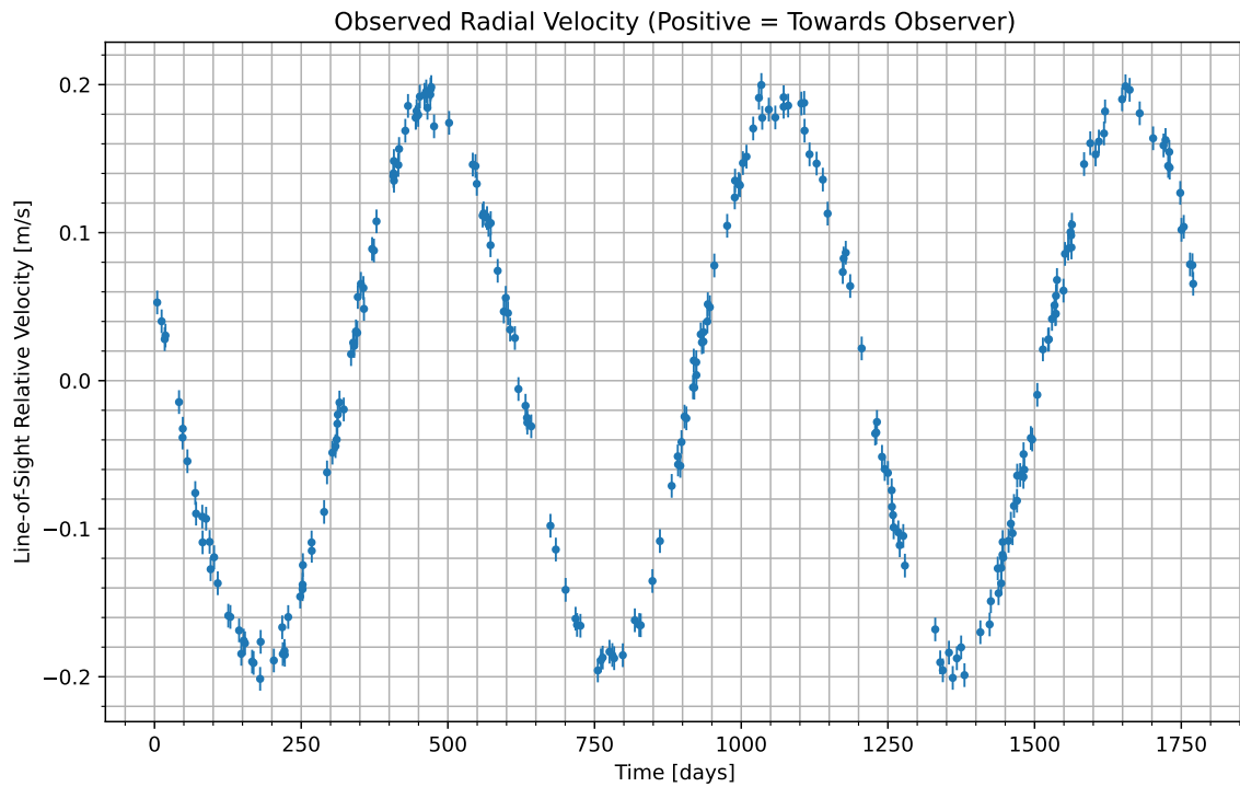
Figure 1: We have isolated the radial velocity of the host star due to the candidate planet. Data begins at UTC 2086-03-19/21:05. Positive values indicate the velocity at which the star is moving towards us; negative indicate the velocity at which it is moving away.
