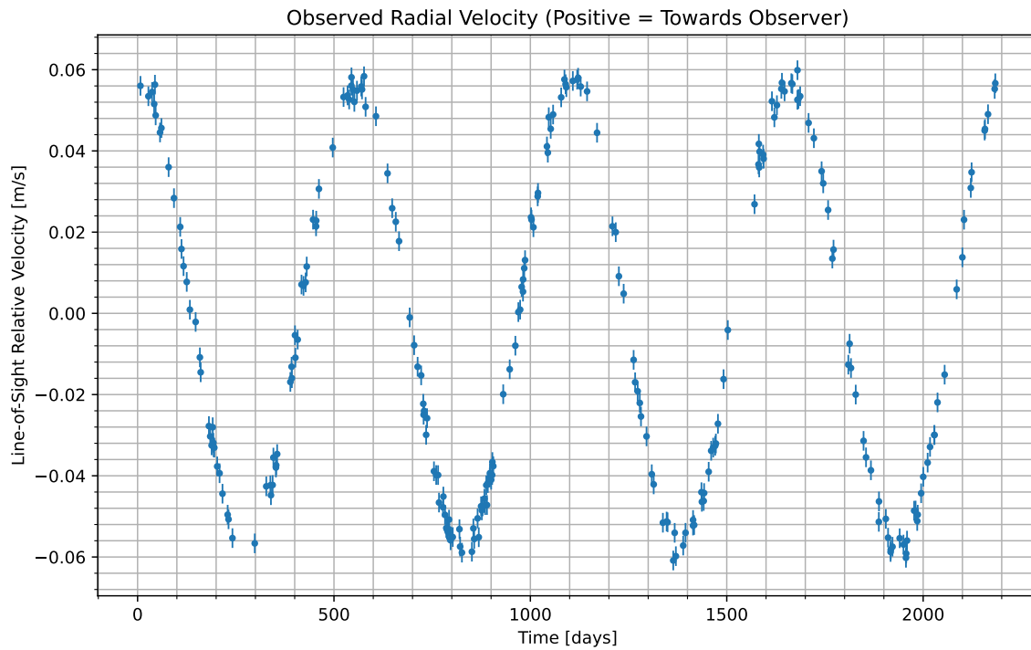
Figure 1: We have isolated the radial velocity of the host star due to the candidate planet. Data begins at UTC 2088-07-27/05:44. Positive values indicate the velocity at which the star is moving towards us; negative indicate the velocity at which it is moving away.
