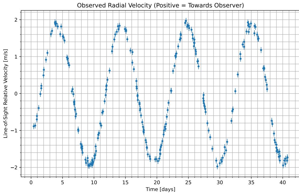
Figure 1: We have isolated the radial velocity of the host star due to the candidate planet. Data begins at UTC 2074-05-13/01:13. Positive values indicate the velocity at which the star is moving towards us; negative indicate the velocity at which it is moving away.
