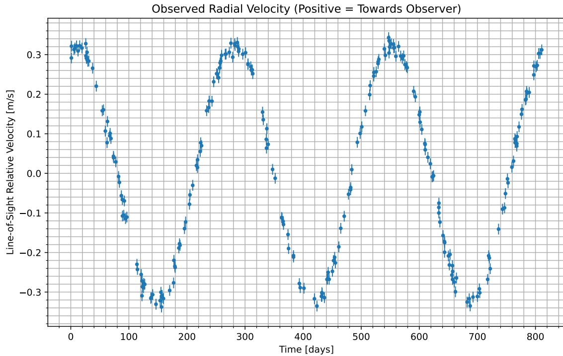
Figure 1: We have isolated the radial velocity of the host star due to the candidate planet. Data begins at UTC 2075-06-22/13:55. Positive values indicate the velocity at which the star is moving towards us; negative indicate the velocity at which it is moving away.
