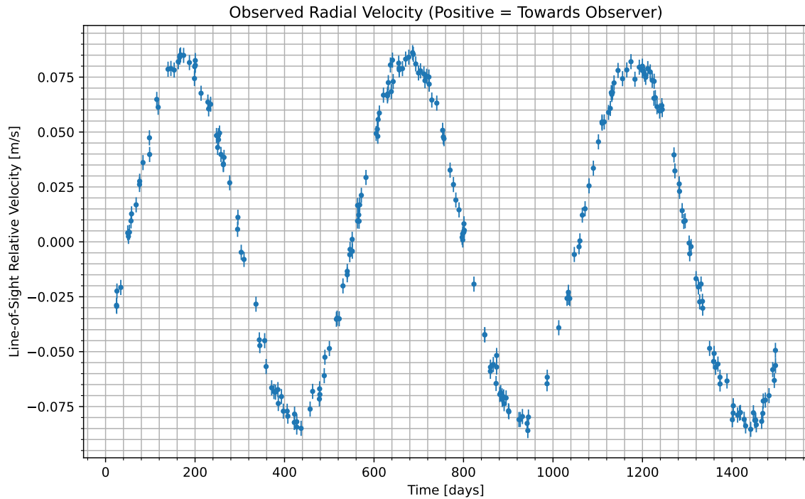
Figure 1: We have isolated the radial velocity of the host star due to the candidate planet. Data begins at UTC 2074-05-12/12:31. Positive values indicate the velocity at which the star is moving towards us; negative indicate the velocity at which it is moving away.
