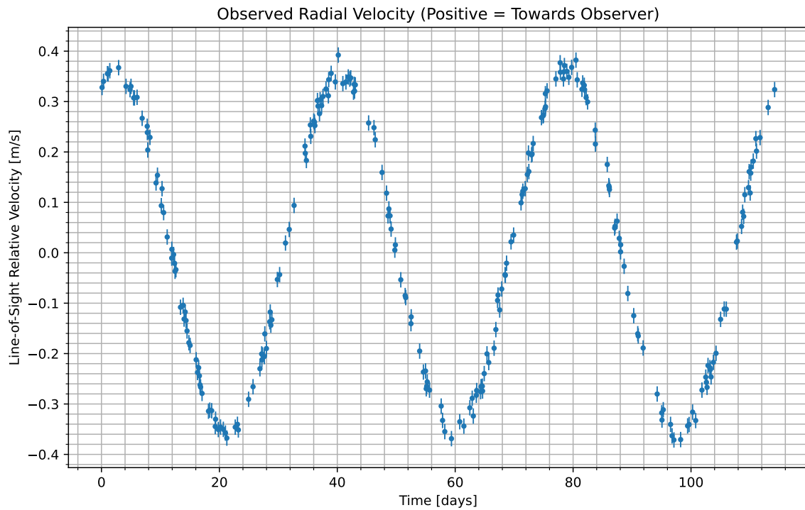
Figure 1: We have isolated the radial velocity of the host star due to the candidate planet. Data begins at UTC 2087-01-12/17:36. Positive values indicate the velocity at which the star is moving towards us; negative indicate the velocity at which it is moving away.
