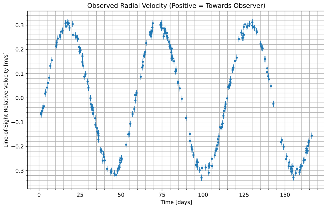
Figure 1: We have isolated the radial velocity of the host star due to the candidate planet. Data begins at UTC 2079-02-25/06:49. Positive values indicate the velocity at which the star is moving towards us; negative indicate the velocity at which it is moving away.
