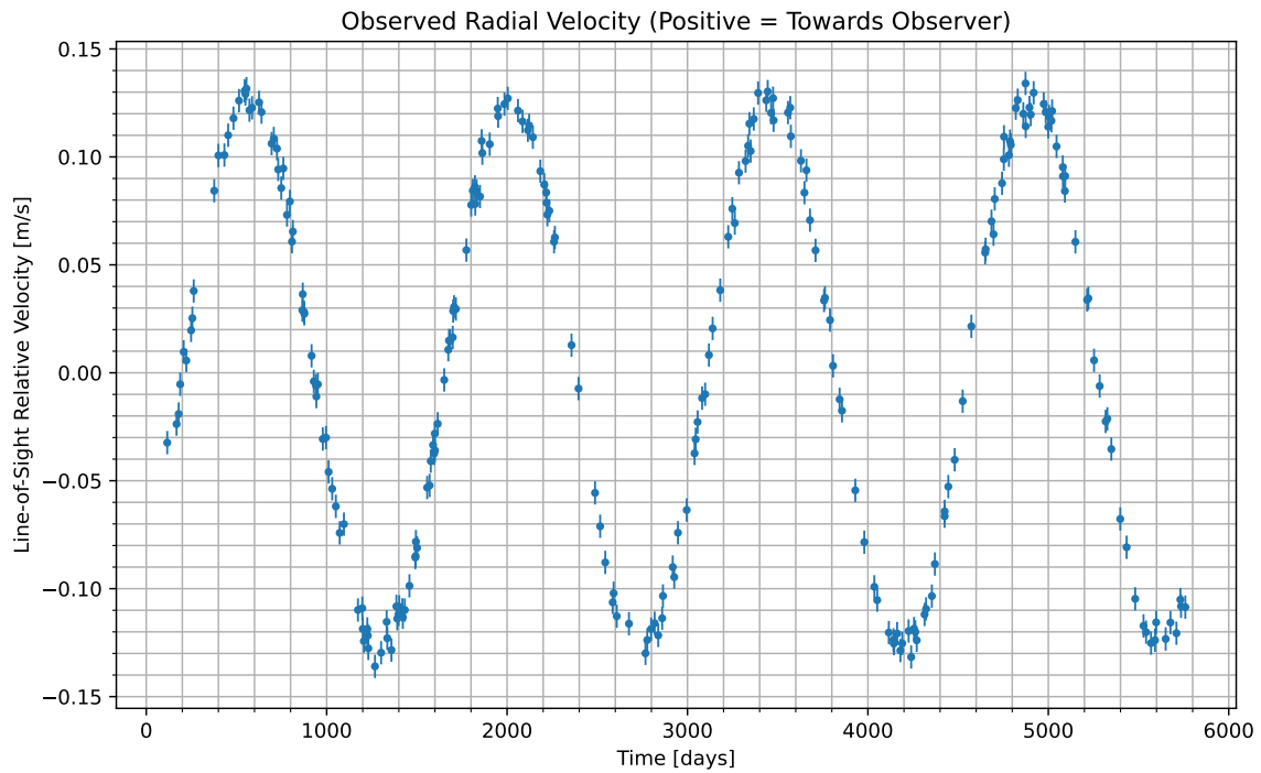
Figure 1: We have isolated the radial velocity of the host star due to the candidate planet. Data begins at UTC 2085-01-02/09:21. Positive values indicate the velocity at which the star is moving towards us; negative indicate the velocity at which it is moving away.
