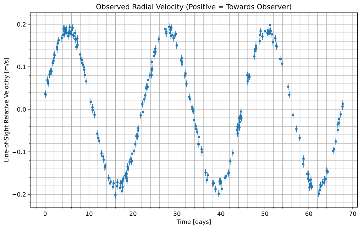
Figure 1: We have isolated the radial velocity of the host star due to the candidate planet. Data begins at UTC 2073-03-04/14:00. Positive values indicate the velocity at which the star is moving towards us; negative indicate the velocity at which it is moving away.
