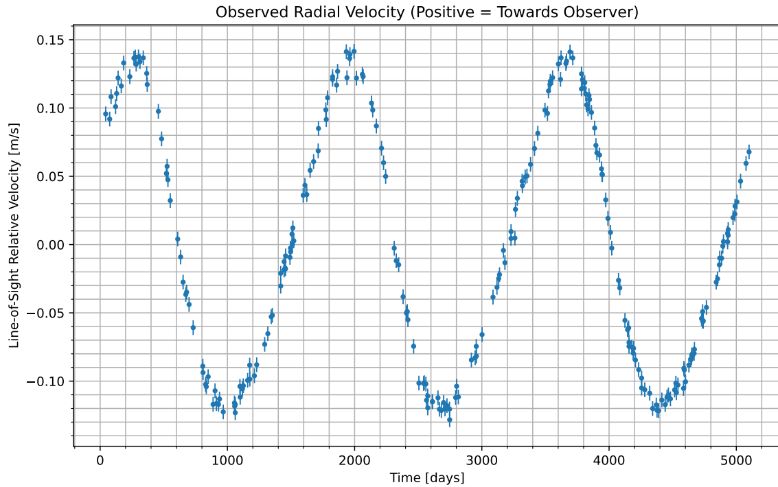
Figure 1: We have isolated the radial velocity of the host star due to the candidate planet. Data begins at UTC 2085-04-09/23:55. Positive values indicate the velocity at which the star is moving towards us; negative indicate the velocity at which it is moving away.
