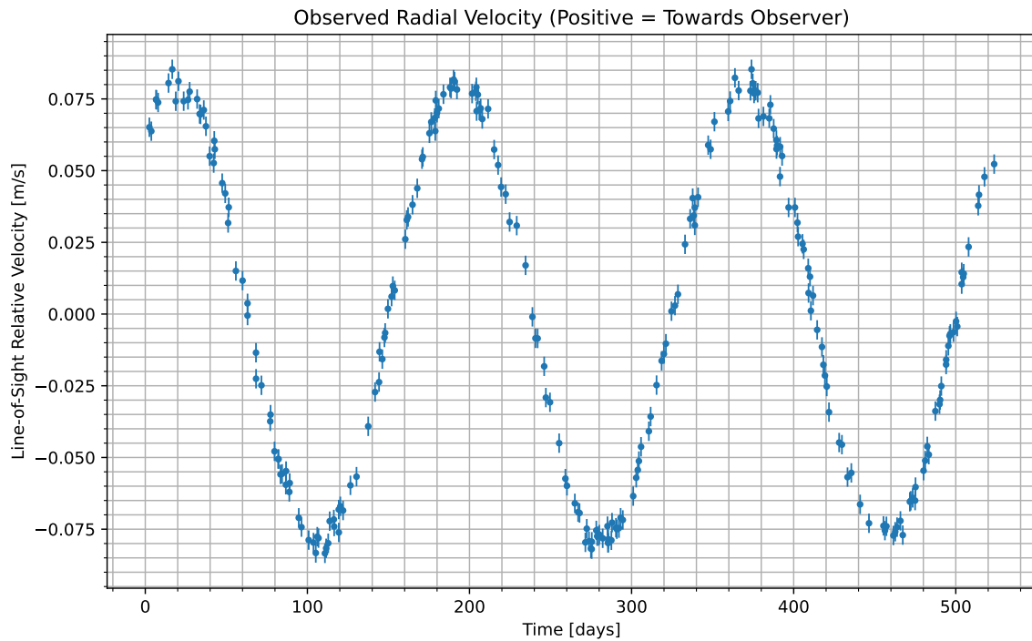
Figure 1: We have isolated the radial velocity of the host star due to the candidate planet. Data begins at UTC 2079-08-14/02:26. Positive values indicate the velocity at which the star is moving towards us; negative indicate the velocity at which it is moving away.
