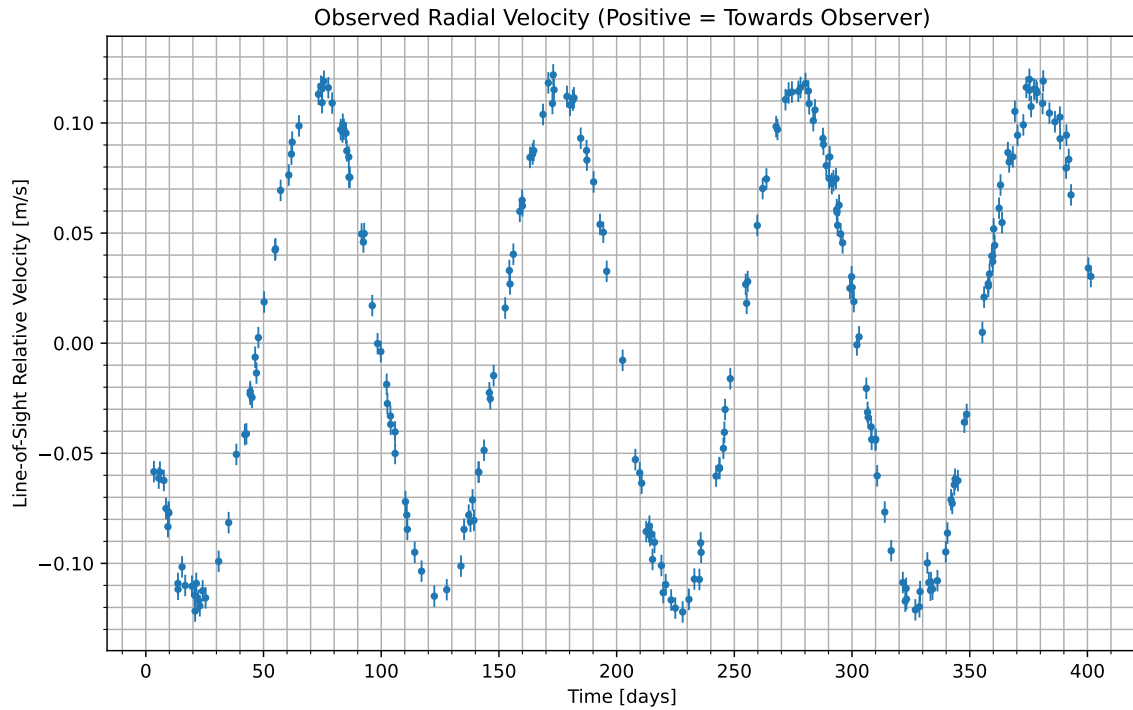
Figure 1: We have isolated the radial velocity of the host star due to the candidate planet. Data begins at UTC 2078-11-03/18:21. Positive values indicate the velocity at which the star is moving towards us; negative indicate the velocity at which it is moving away.
