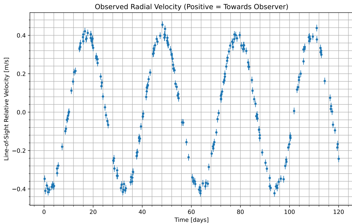
Figure 1: We have isolated the radial velocity of the host star due to the candidate planet. Data begins at UTC 2096-11-15/18:57. Positive values indicate the velocity at which the star is moving towards us; negative indicate the velocity at which it is moving away.
