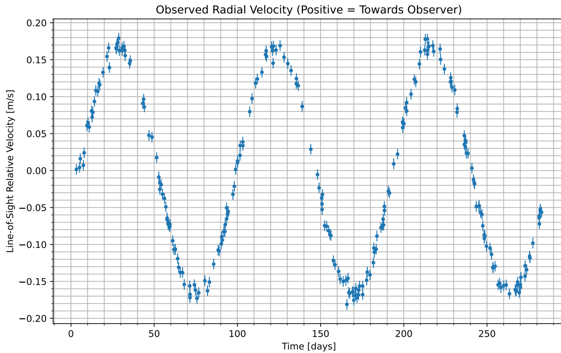
Figure 1: We have isolated the radial velocity of the host star due to the candidate planet. Data begins at UTC 2069-11-02/14:05. Positive values indicate the velocity at which the star is moving towards us; negative indicate the velocity at which it is moving away.
