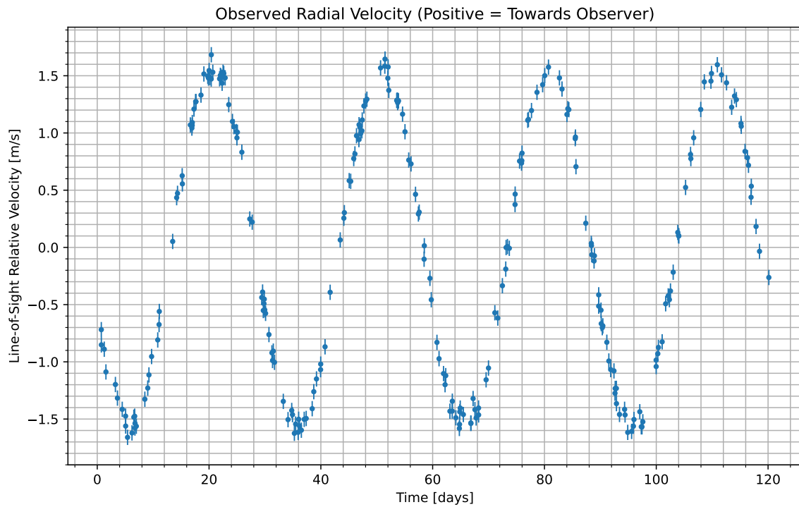
Figure 1: We have isolated the radial velocity of the host star due to the candidate planet. Data begins at UTC 2070-12-23/04:35. Positive values indicate the velocity at which the star is moving towards us; negative indicate the velocity at which it is moving away.
