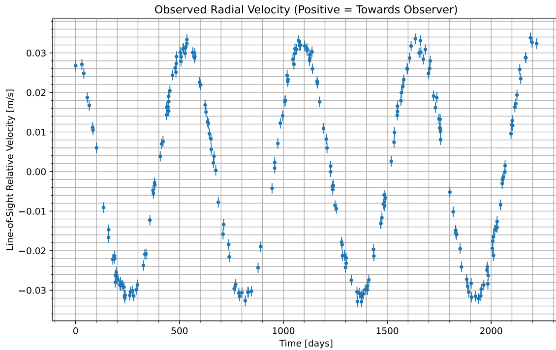
Figure 1: We have isolated the radial velocity of the host star due to the candidate planet. Data begins at UTC 2081-09-24/05:22. Positive values indicate the velocity at which the star is moving towards us; negative indicate the velocity at which it is moving away.
