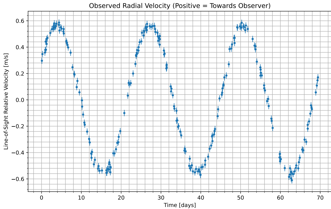
Figure 1: We have isolated the radial velocity of the host star due to the candidate planet. Data begins at UTC 2085-06-08/13:57. Positive values indicate the velocity at which the star is moving towards us; negative indicate the velocity at which it is moving away.
