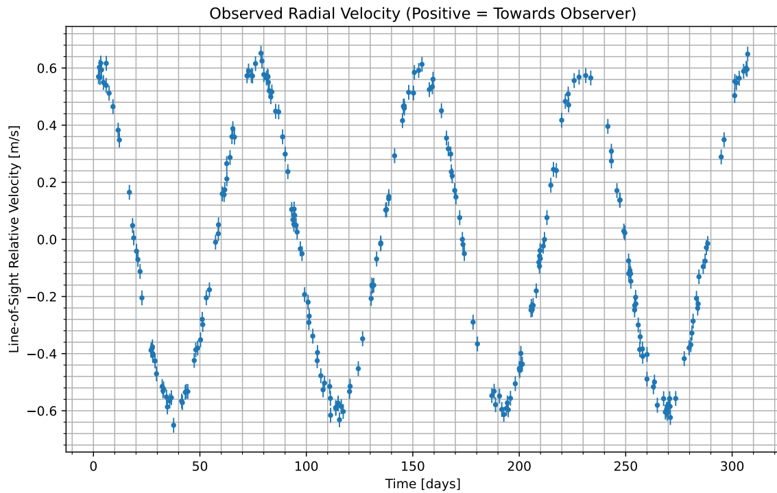
Figure 1: We have isolated the radial velocity of the host star due to the candidate planet. Data begins at UTC 2078-12-24/06:56. Positive values indicate the velocity at which the star is moving towards us; negative indicate the velocity at which it is moving away.
