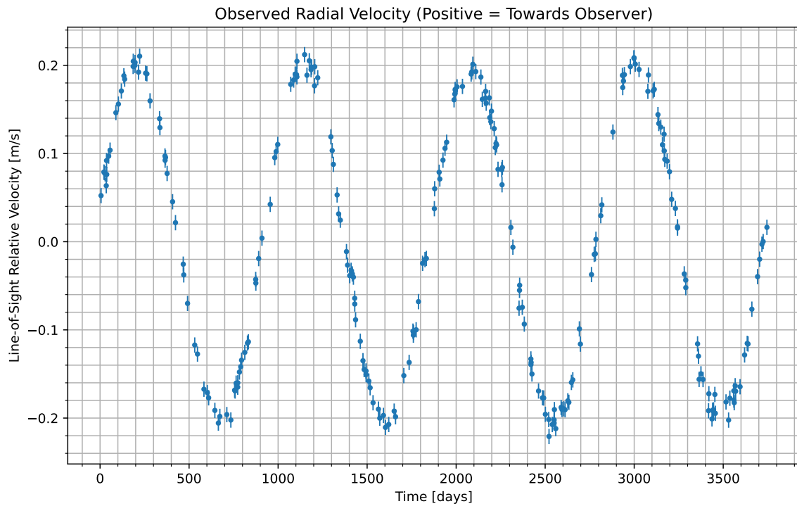
Figure 1: We have isolated the radial velocity of the host star due to the candidate planet. Data begins at UTC 2062-09-16/05:41. Positive values indicate the velocity at which the star is moving towards us; negative indicate the velocity at which it is moving away.
