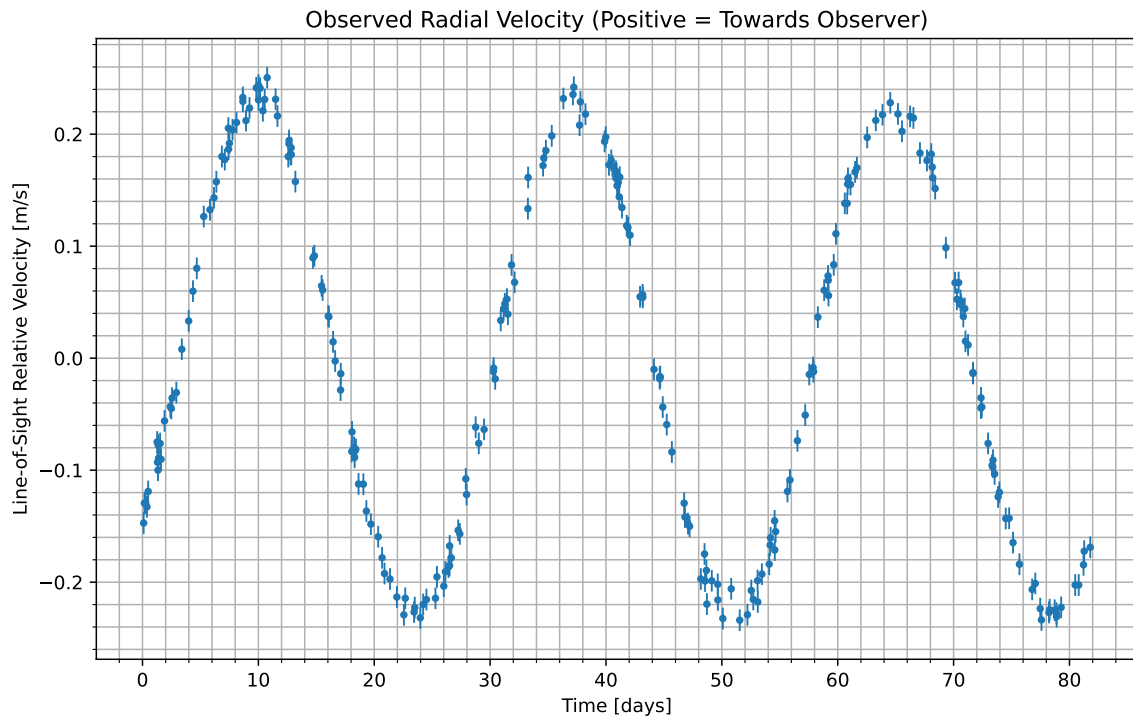
Figure 1: We have isolated the radial velocity of the host star due to the candidate planet. Data begins at UTC 2072-07-15/04:09. Positive values indicate the velocity at which the star is moving towards us; negative indicate the velocity at which it is moving away.
