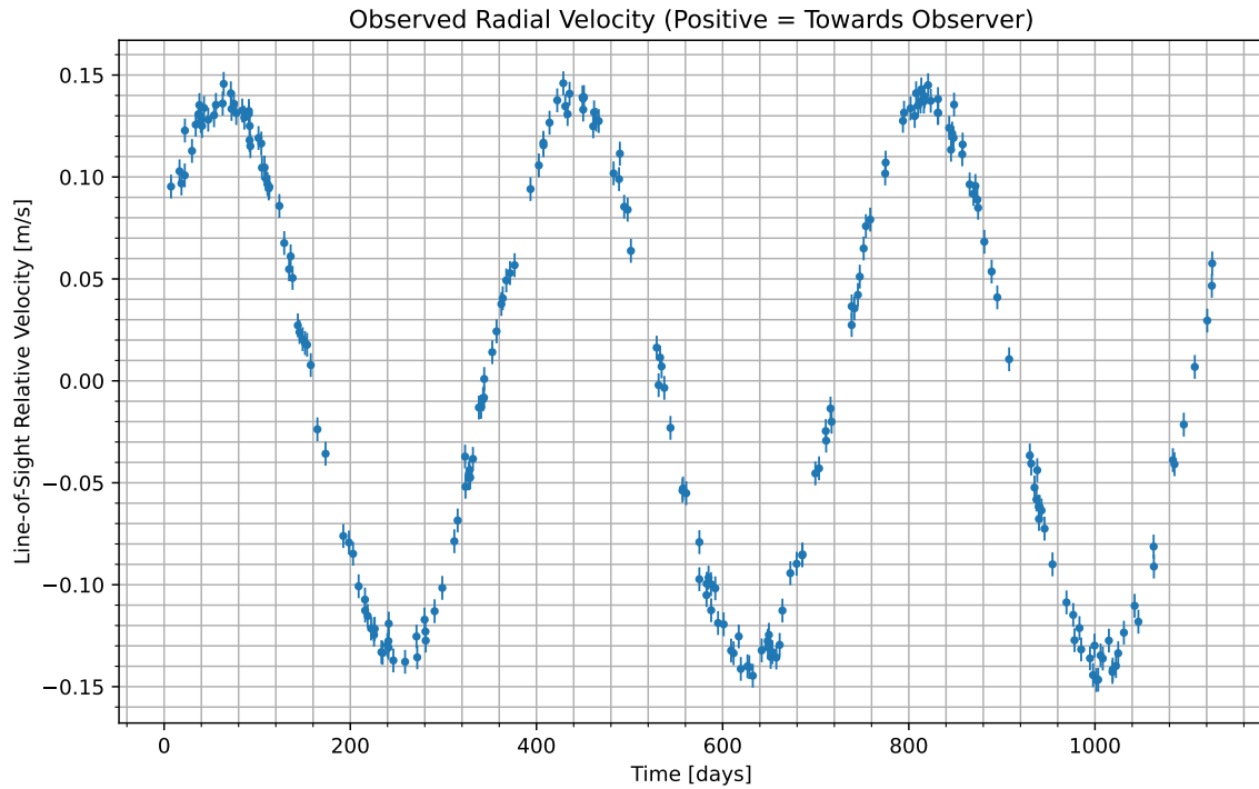
Figure 1: We have isolated the radial velocity of the host star due to the candidate planet. Data begins at UTC 2097-09-27/10:56. Positive values indicate the velocity at which the star is moving towards us; negative indicate the velocity at which it is moving away.
