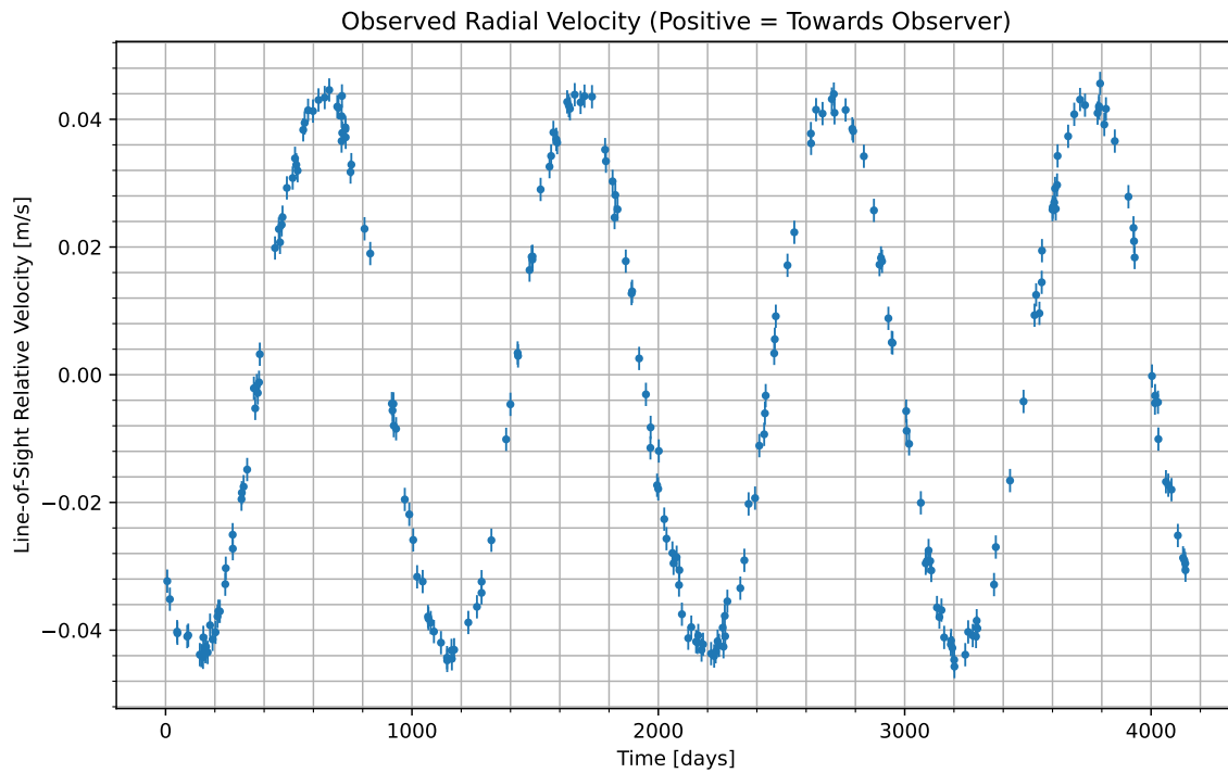
Figure 1: We have isolated the radial velocity of the host star due to the candidate planet. Data begins at UTC 2075-02-09/11:10. Positive values indicate the velocity at which the star is moving towards us; negative indicate the velocity at which it is moving away.
