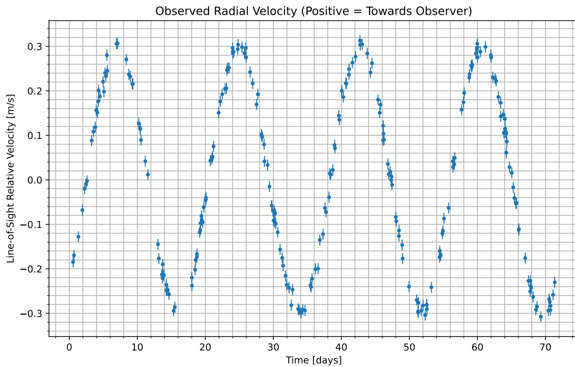
Figure 1: We have isolated the radial velocity of the host star due to the candidate planet. Data begins at UTC 2087-08-03/17:10. Positive values indicate the velocity at which the star is moving towards us; negative indicate the velocity at which it is moving away.
