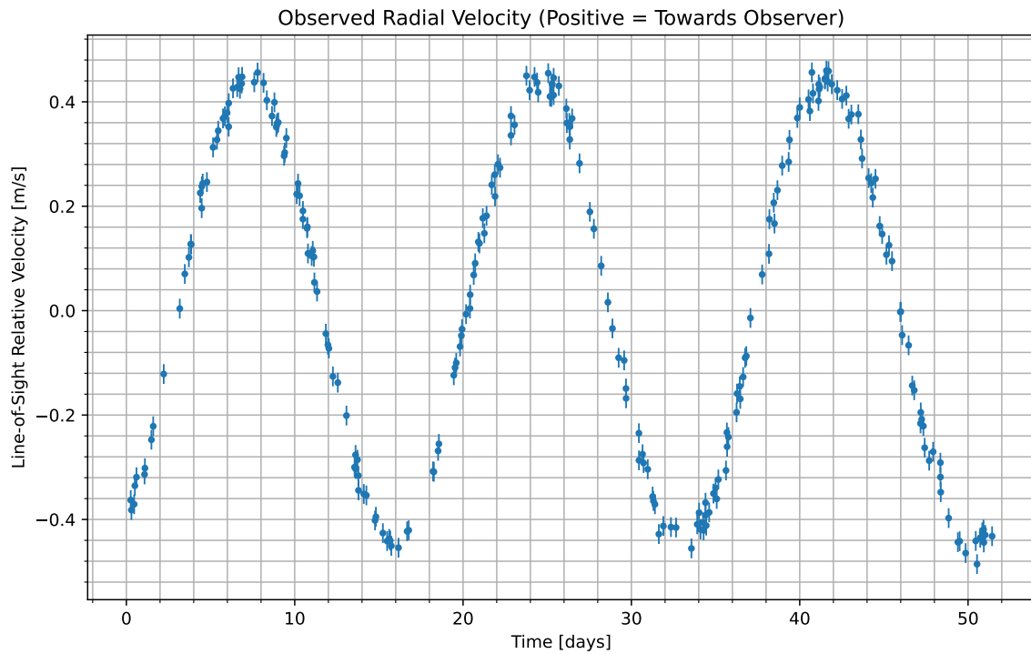
Figure 1: We have isolated the radial velocity of the host star due to the candidate planet. Data begins at UTC 2075-07-29/22:12. Positive values indicate the velocity at which the star is moving towards us; negative indicate the velocity at which it is moving away.
