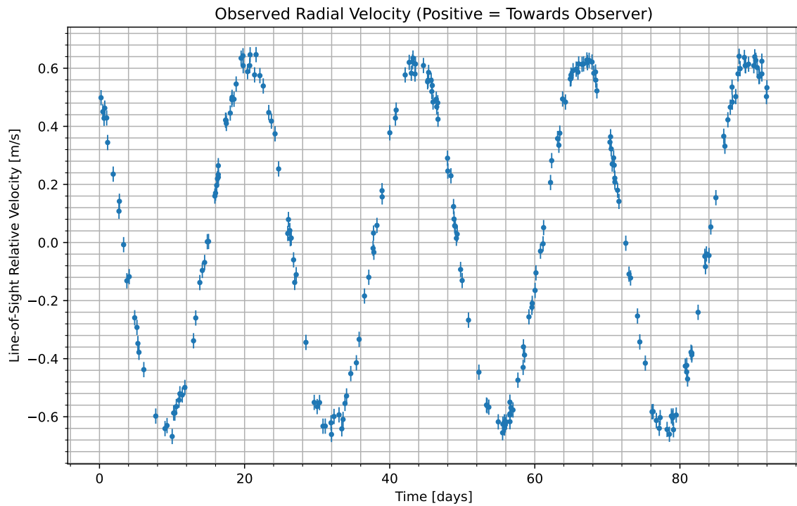
Figure 1: We have isolated the radial velocity of the host star due to the candidate planet. Data begins at UTC 2098-04-02/17:31. Positive values indicate the velocity at which the star is moving towards us; negative indicate the velocity at which it is moving away.
