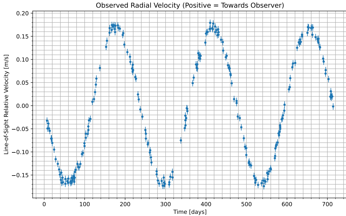
Figure 1: We have isolated the radial velocity of the host star due to the candidate planet. Data begins at UTC 2094-10-31/20:23. Positive values indicate the velocity at which the star is moving towards us; negative indicate the velocity at which it is moving away.
