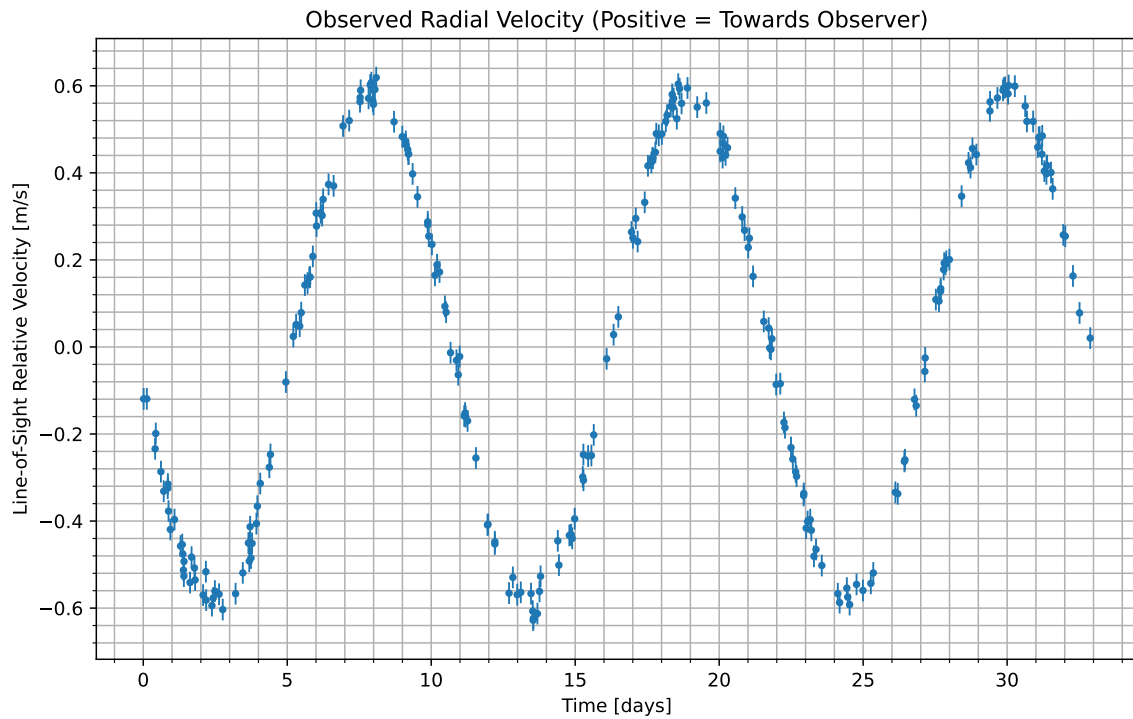
Figure 1: We have isolated the radial velocity of the host star due to the candidate planet. Data begins at UTC 2076-07-20/15:28. Positive values indicate the velocity at which the star is moving towards us; negative indicate the velocity at which it is moving away.
