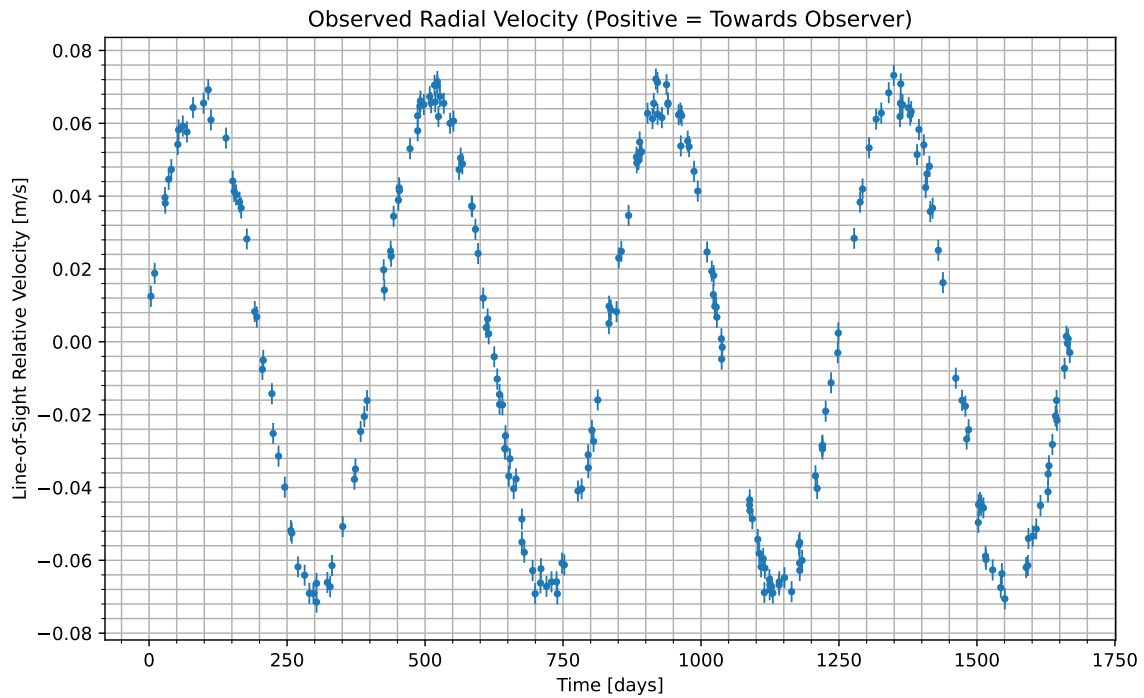
Figure 1: We have isolated the radial velocity of the host star due to the candidate planet. Data begins at UTC 2067-03-01/02:58. Positive values indicate the velocity at which the star is moving towards us; negative indicate the velocity at which it is moving away.
