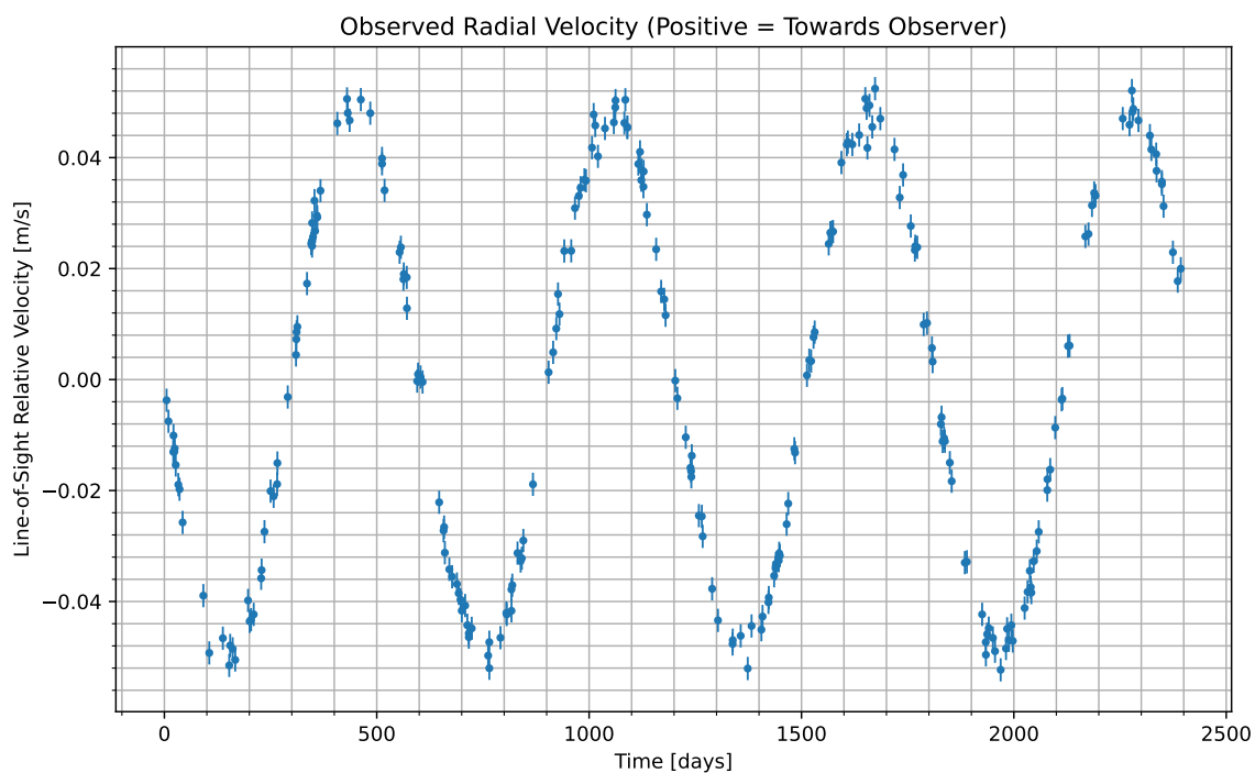
Figure 1: We have isolated the radial velocity of the host star due to the candidate planet. Data begins at UTC 2090-10-06/18:53. Positive values indicate the velocity at which the star is moving towards us; negative indicate the velocity at which it is moving away.
