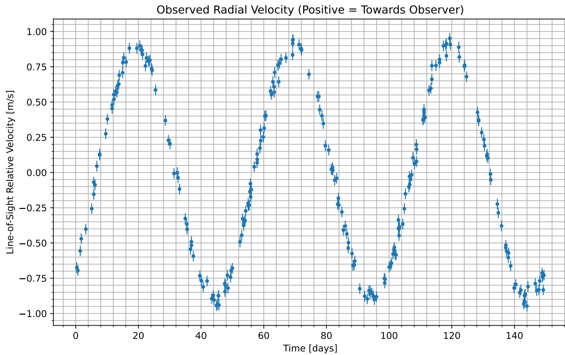
Figure 1: We have isolated the radial velocity of the host star due to the candidate planet. Data begins at UTC 2092-04-03/12:01. Positive values indicate the velocity at which the star is moving towards us; negative indicate the velocity at which it is moving away.
