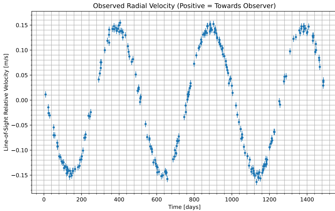
Figure 1: We have isolated the radial velocity of the host star due to the candidate planet. Data begins at UTC 2088-02-08/19:26. Positive values indicate the velocity at which the star is moving towards us; negative indicate the velocity at which it is moving away.
