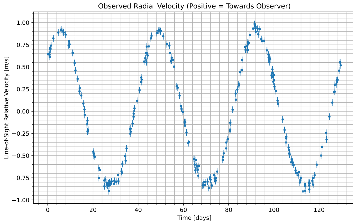
Figure 1: We have isolated the radial velocity of the host star due to the candidate planet. Data begins at UTC 2082-07-15/10:03. Positive values indicate the velocity at which the star is moving towards us; negative indicate the velocity at which it is moving away.
