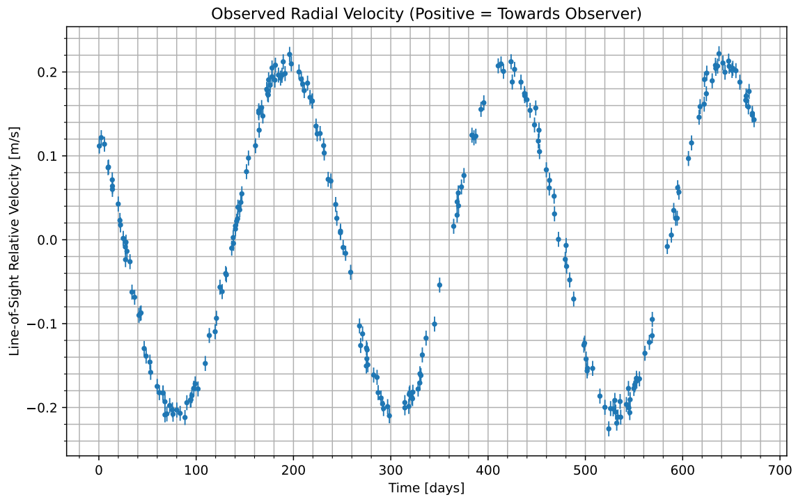
Figure 1: We have isolated the radial velocity of the host star due to the candidate planet. Data begins at UTC 2069-08-20/07:59. Positive values indicate the velocity at which the star is moving towards us; negative indicate the velocity at which it is moving away.
