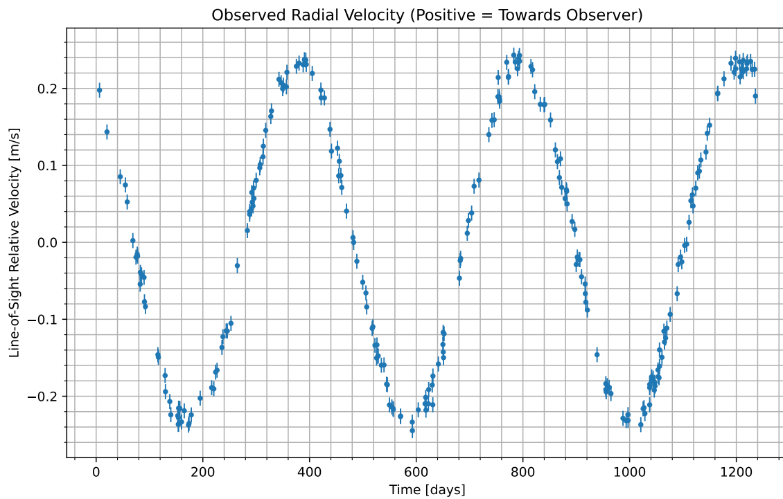
Figure 1: We have isolated the radial velocity of the host star due to the candidate planet. Data begins at UTC 2094-03-07/11:17. Positive values indicate the velocity at which the star is moving towards us; negative indicate the velocity at which it is moving away.
