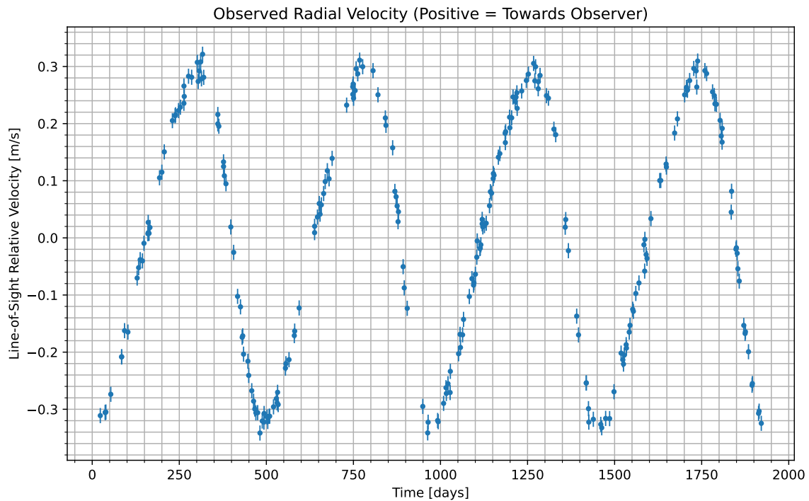
Figure 1: We have isolated the radial velocity of the host star due to the candidate planet. Data begins at UTC 2095-07-02/07:58. Positive values indicate the velocity at which the star is moving towards us; negative indicate the velocity at which it is moving away.
