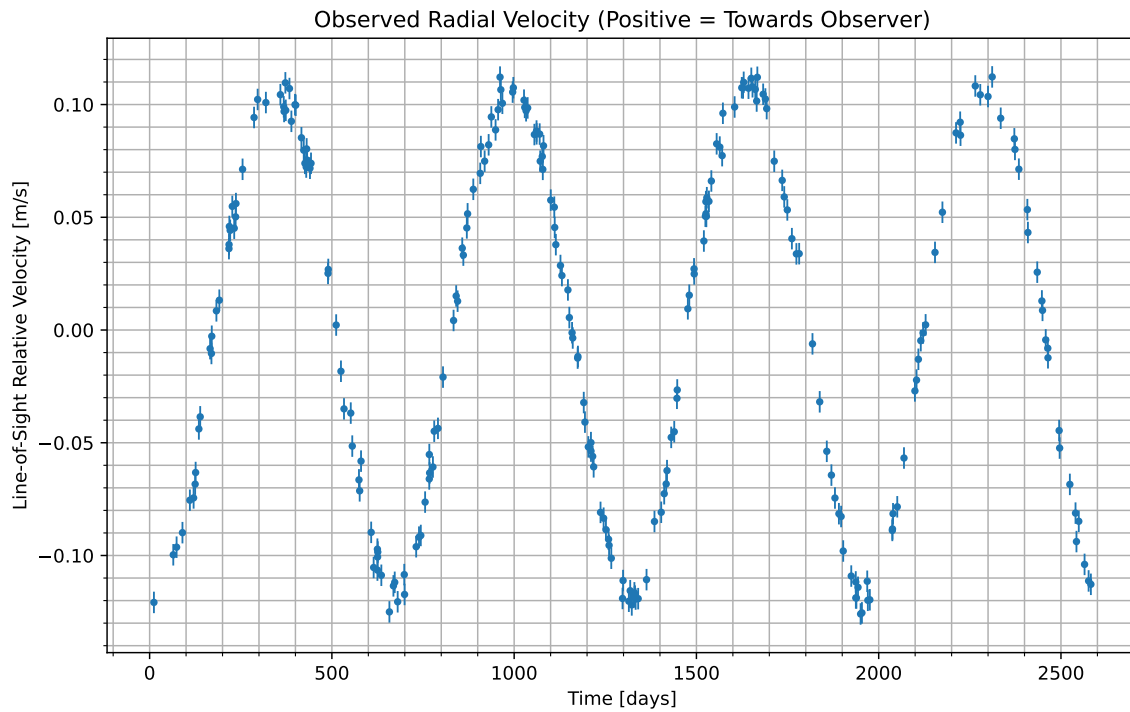
Figure 1: We have isolated the radial velocity of the host star due to the candidate planet. Data begins at UTC 2075-10-03/10:47. Positive values indicate the velocity at which the star is moving towards us; negative indicate the velocity at which it is moving away.
