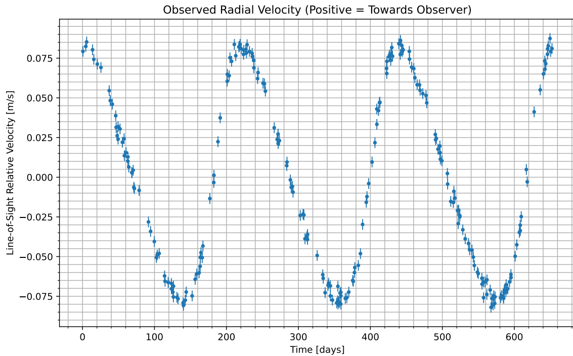
Figure 1: We have isolated the radial velocity of the host star due to the candidate planet. Data begins at UTC 2095-02-06/01:13. Positive values indicate the velocity at which the star is moving towards us; negative indicate the velocity at which it is moving away.
